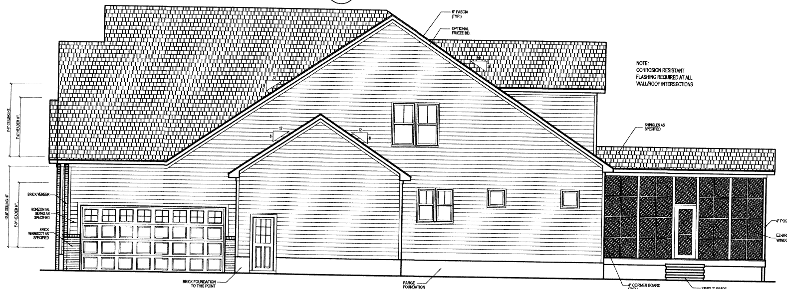
2 LEFT ELEVATION SCALE: 3/16" = 1'-0"
