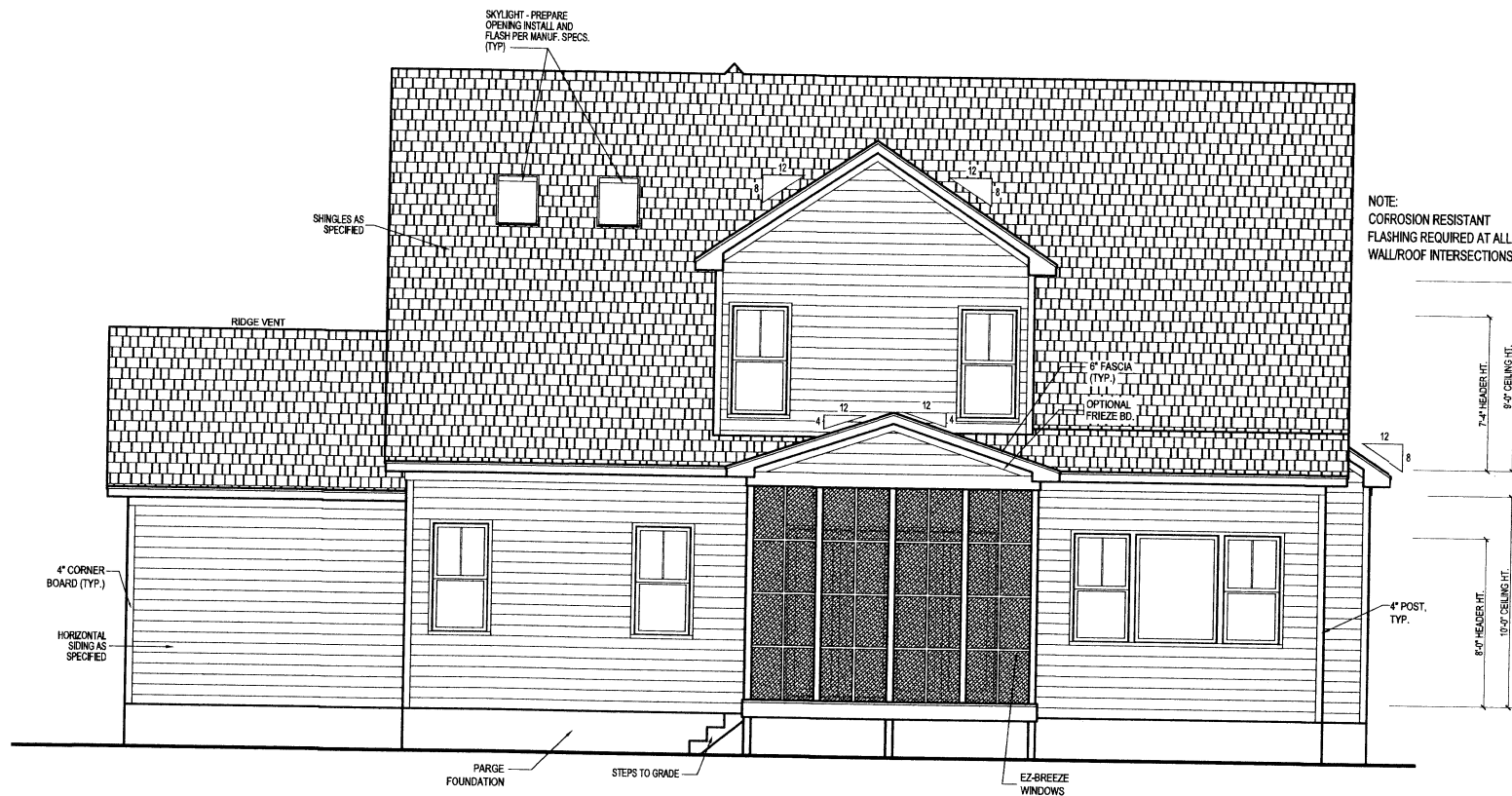
4 REAR ELEVATION SCALE: 1/4" = 1'-0"
