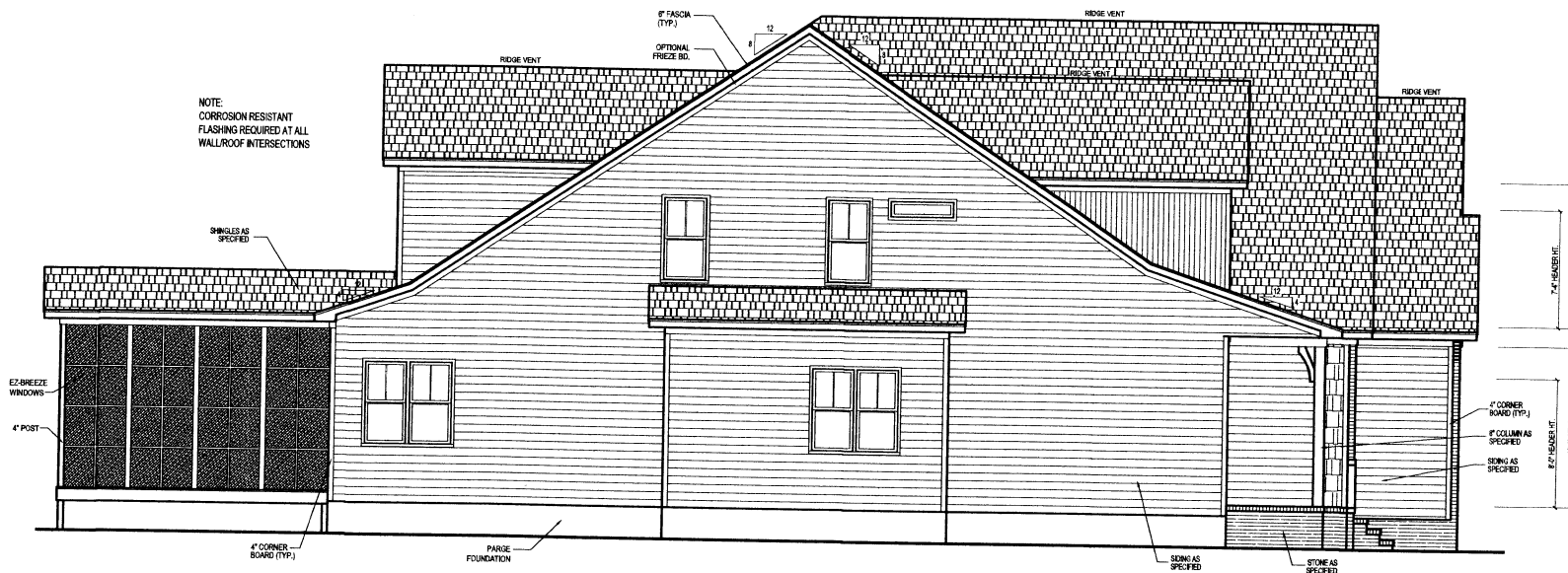
3 RIGHT ELEVATION SCALE: 3/16" = 1'-0"
